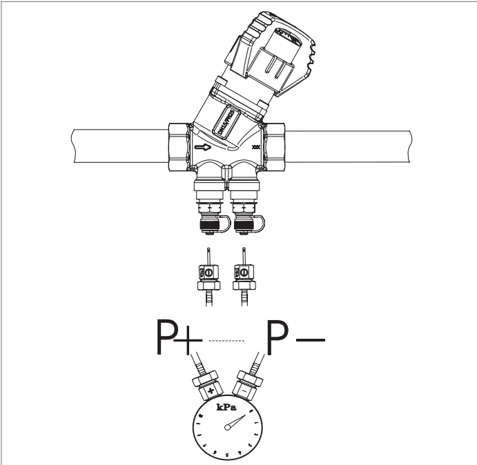
Measurement of the differential pressure ( \Delta p ) across the valve
