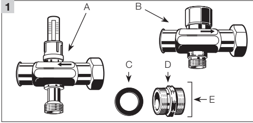
Model 2890-4
