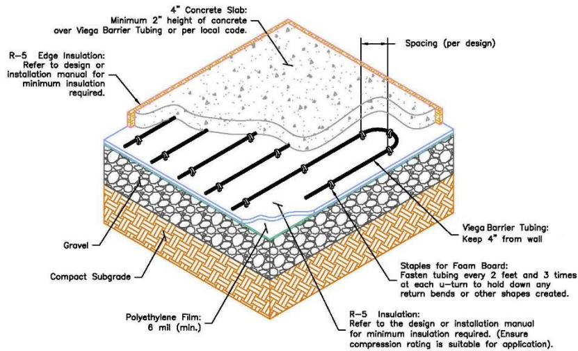
Figure 6 In-Slab – Foamboard Staples
