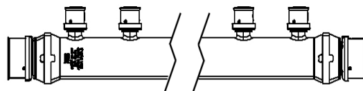
FIGURE 12 VIEGA PureFlow PRESS POLYMER MANIFOLD
