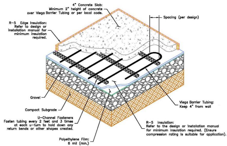
Figure 7 In-Slab – U-Channel
