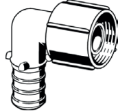
Viega PureFlow Crimp 90° lavatory elbow, PolyAlloy, Model V5255
